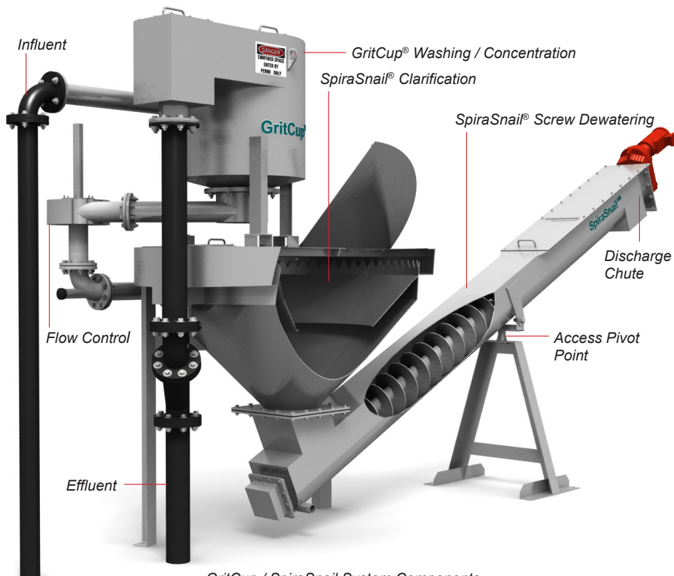
GritCup / SpiraSnail System Components
